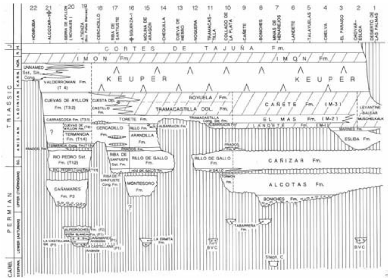
FIGURE 3 | Correlation line I-I' along the Iberian Ranges and part of the Central System. Data from the following sources: 1 to 9, López-Gómez and Arche, 1993, 1994; 10, De las Llanderas, 1984; 11, 12 and 14, Pérez-Arlucea, 1987; 13, López-Gómez, 1985; 15, Ramos, 1979; 16 and 21, IGME, 1987; 17 and 18, García-Gil, 1994; 19 and 20, Hernando, 1977; 22, Vázquez, 1981.
