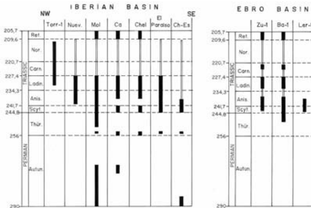
FIGURE 7 | Syn-rift phases (wide, black lines) and post-rift phases (narrow, white lines) for the same sections in figure 6. Note the short-lived, multiphase syn-rift phases. From Vargas, 2002 and Vargas et al., 2004.
